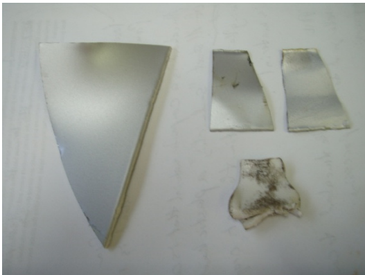
Figure 1: Separation of aluminum skin from plastic core
