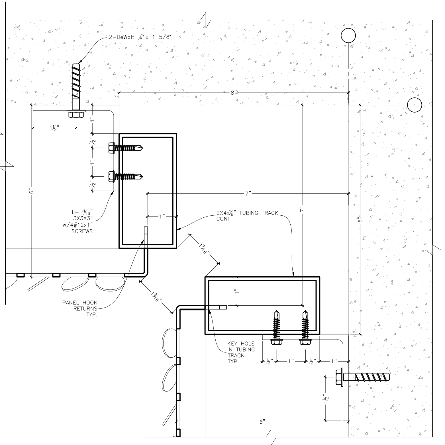
2 D3 DETAIL SCALE 6"=1'-0" SCB REF.: N/A
