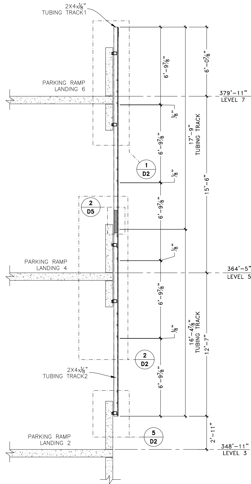
1 SECTION 4.1 SCALE 3/16"=1'-0" ARCH. REF.: N/A
