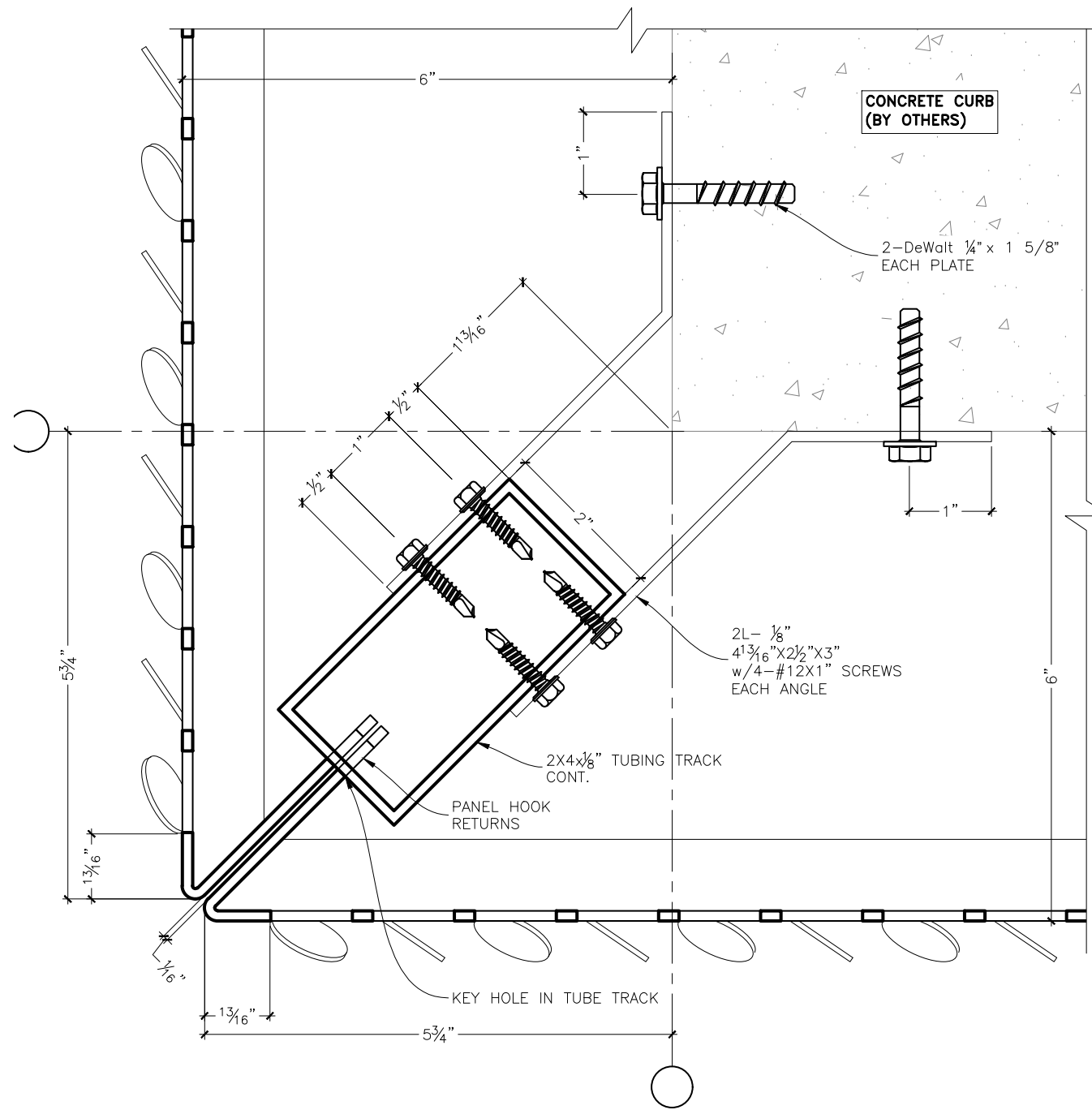
1 D3 DETAIL SCALE 6"=1'-0" SCB REF.: N/A
